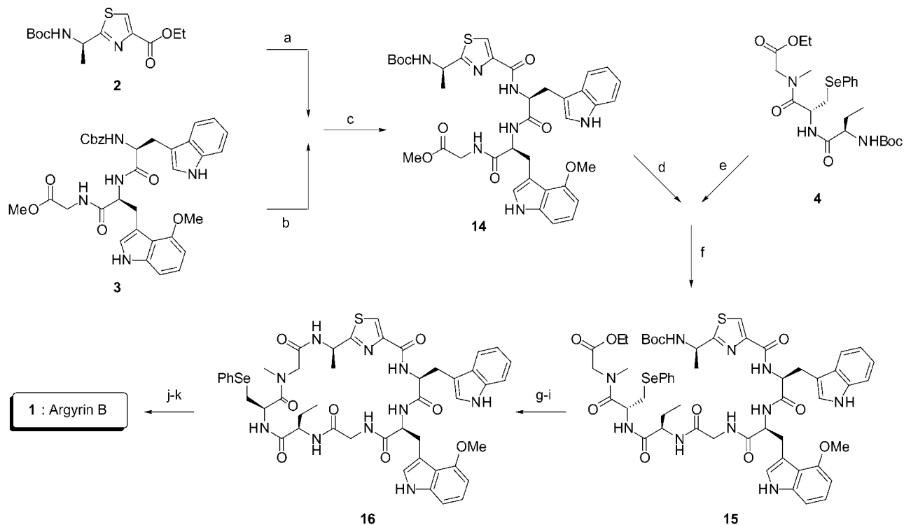
Scheme 4. Synthesis of Argirin B a
