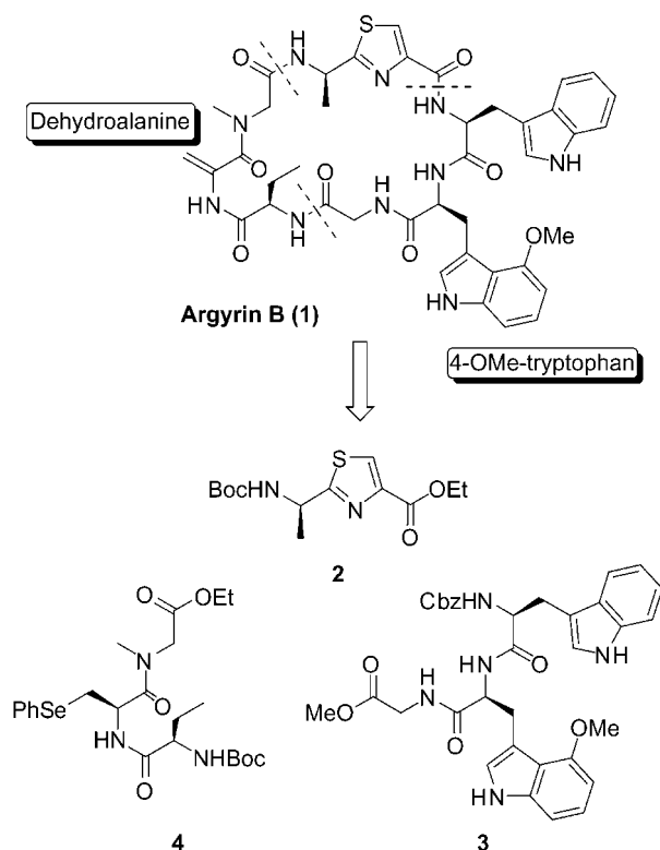
Figure 1. Structure and retrosynthetic analysis of Argyrin B.
