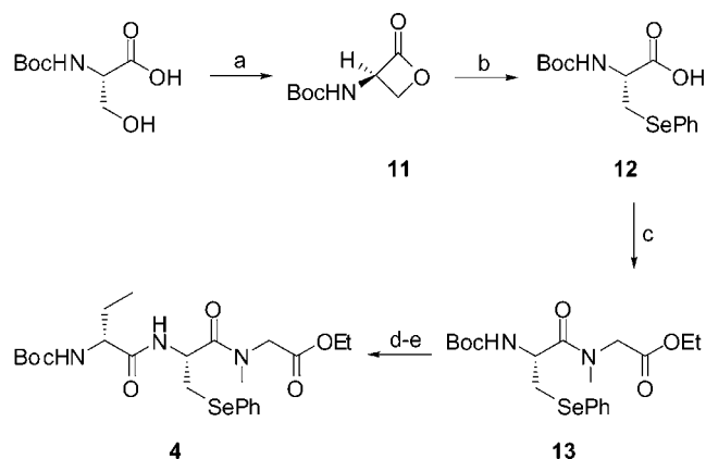
Scheme 3. Synthesis of Fragment 4 a
